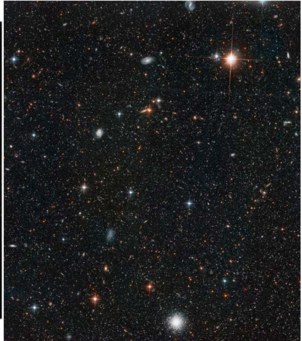
Halo stars
