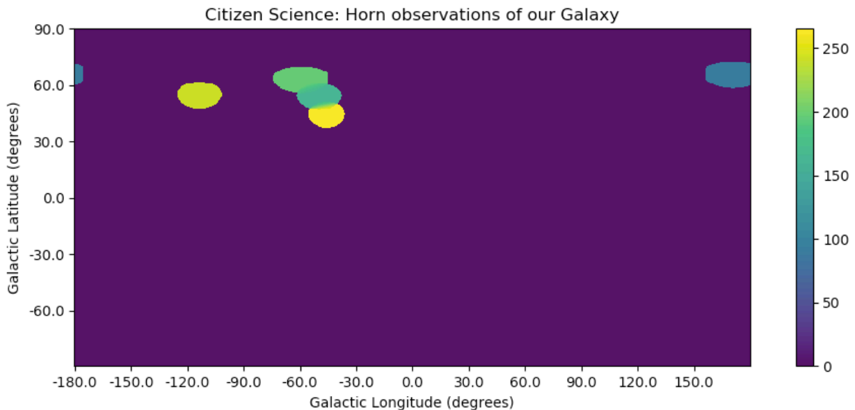
Figure 6: Integrated Intensity Map (Kelvins-km/sec) on a Galactic Longitude, Latitude Map. This is a whole sky map with X axis of Galactic Longitude and Y axis is the Galactic Latitude. The color indicates the signal strength.
