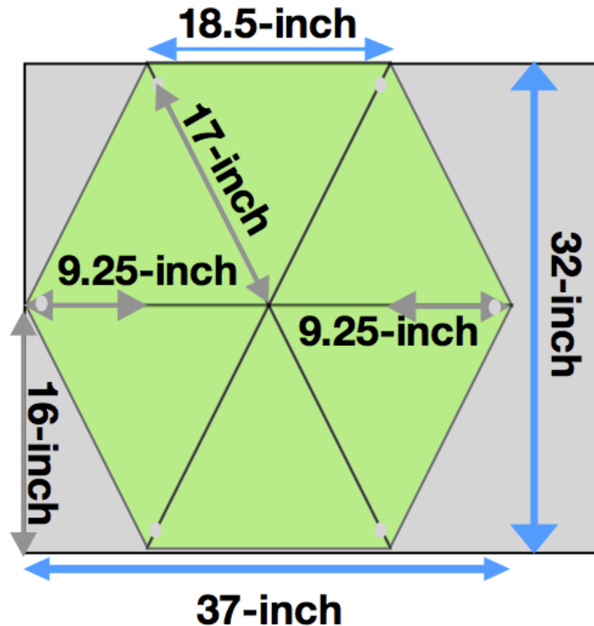
Figure 10: Cone Lid Construction guide for creating a large foam hexagon. The part is created from 1/3 of a 8 ft sheet of 3/4 inch thick foam insulation. The largest dimension is 37 inches and the hexagon is 32 inches wide in three directions. The support legs feed through 6 holes on the edge of the hexagon. The holes are 1-inch in diameter, 17-inch from the center of the hexagon.
