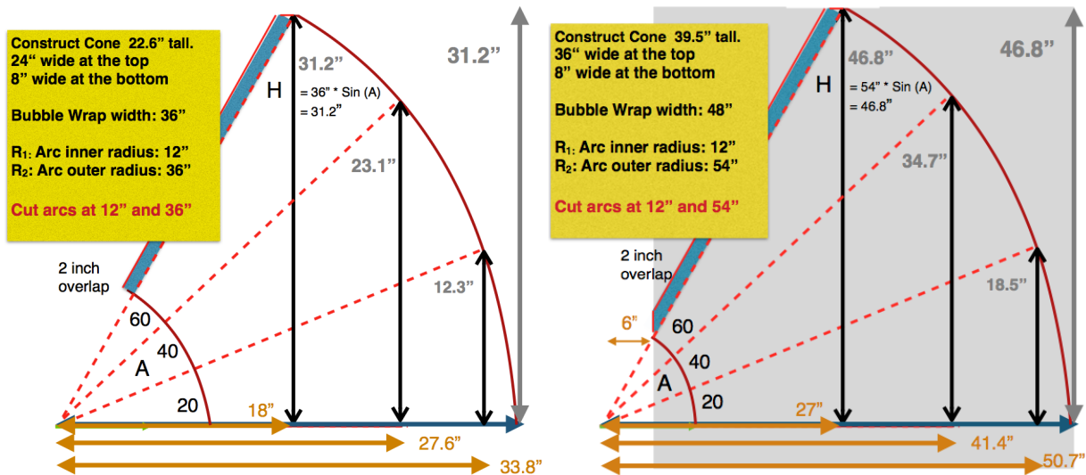
Figure 14: Bubble wrap measurements for constructing a 24 inch wide cone (left) and 36 inch wide cone (right). These measurements are from a point defining the center of the arcs to be cut. For the 24 inch cone, the point is at the edge of the bubble wrap. For the 36 inch diameter cone, the point is 6 inches off of the bubble wrap. To draw the arcs, tape the bubble wrap to the floor and mark the center point on the floor. (Note the 24 inch cone leg positions happen to each have only 3 digits: 12.3", 23.1" and 31.2")
