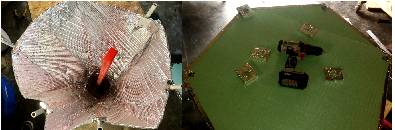
Figure 12: Horn attached to reducer, but no cap yet. At right the horn lid is being attached to the legs. Because of the symmetry of the horn, the lid can act as a table, for light weight items.
